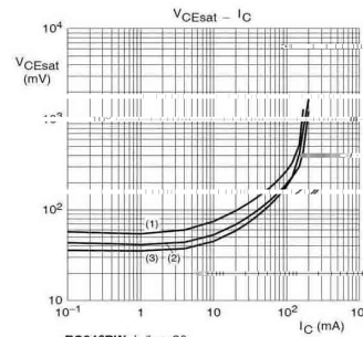
BC846BW ; I_C/I_B = 20 . (1) T_{amb} = 150^{\circ}C . (2) T_{amb} = 25^{\circ}C . (3) T_{amb} = -55^{\circ}C .
